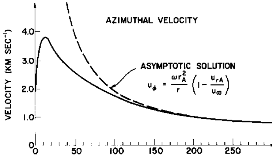
Figure 20: Comparison of asymptotic form for azimuthal flow velocity of solar wind with Weber-Davis solution.
