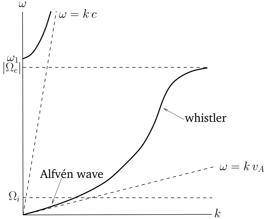
Figure 10: Dispersion relation for a right-handed wave propagating parallel to the magnetic field in a magnetized plasma.
