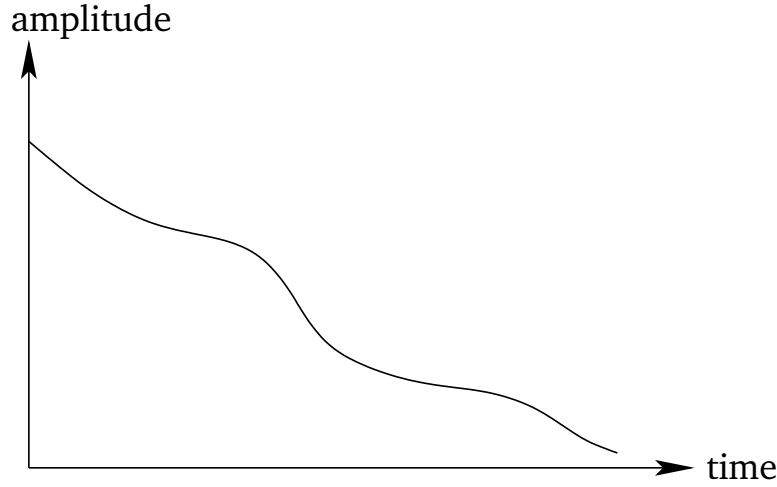
Figure 36: Nonlinear Landau damping.
