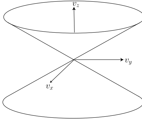
Figure 2: Loss cone in velocity space. The particles lying inside the cone are not reflected by the magnetic field.
