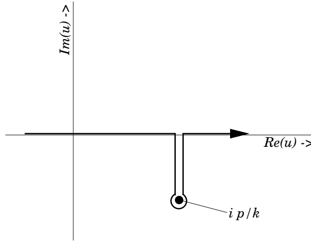
Figure 33: The Bromwich contour for Landau damping.
