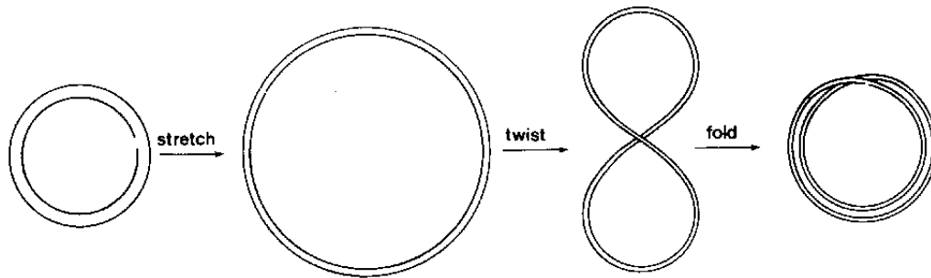
Figure 23: The stretch-twist-fold cycle of a fast dynamo.
