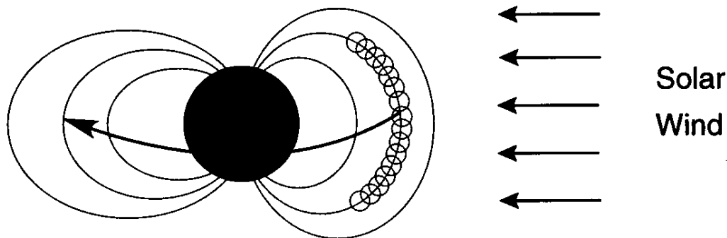
Figure 4: The distortion of the Earth's magnetic field by the solar wind.
