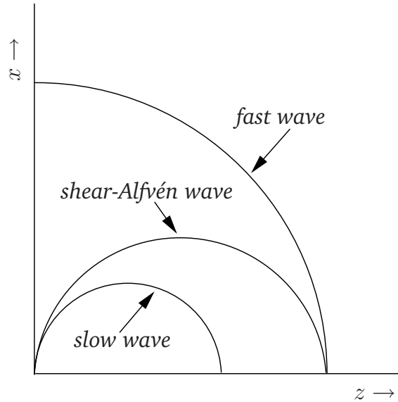
Figure 16: Phase velocities of the three MHD waves in the x - z plane.
