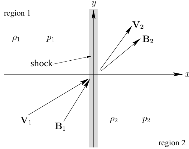
Figure 28: A planar shock.
