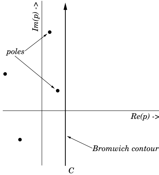
Figure 31: The Bromwich contour.
