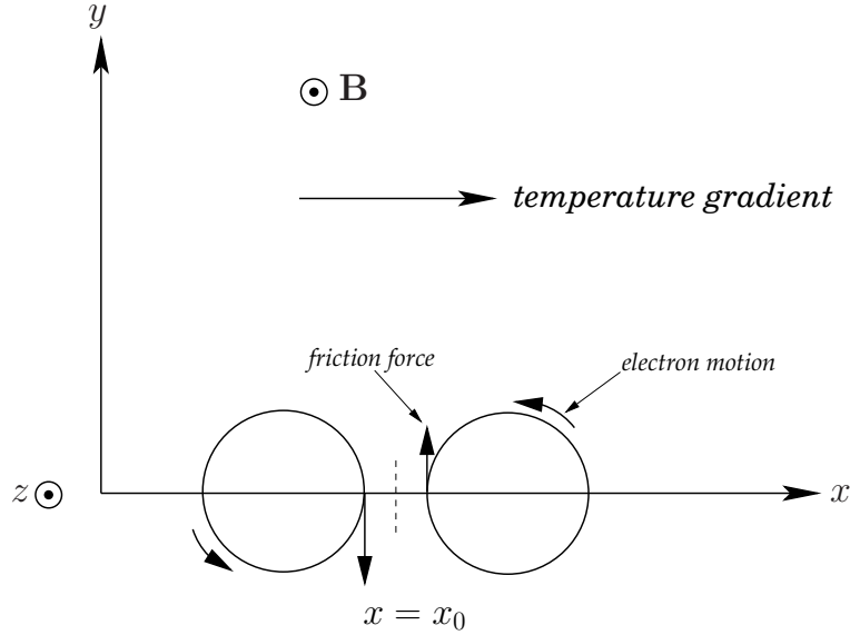
Figure 5: Origin of the perpendicular thermal force in a magnetized plasma.
