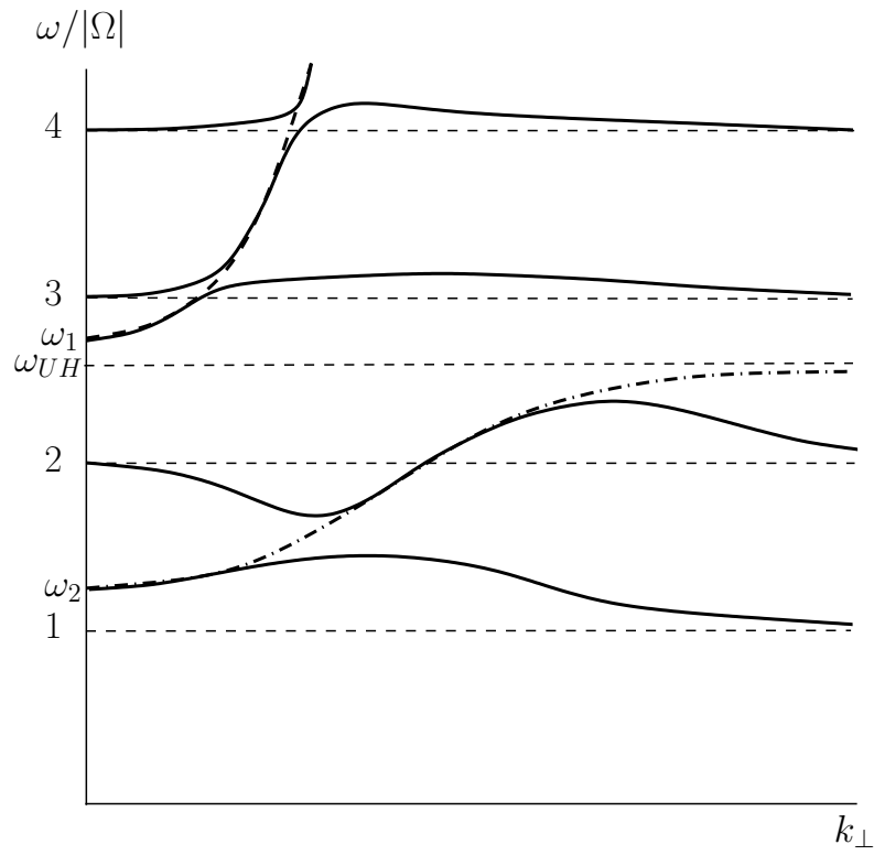
Figure 39: Dispersion relation for electron Bernstein waves in a warm plasma. The dashed line indicates the cold plasma extraordinary mode.
