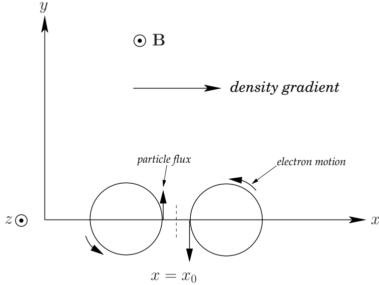
Figure 7: Origin of the diamagnetic velocity in a magnetized plasma.
