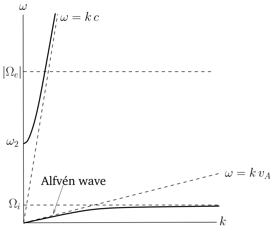
Figure 13: Dispersion relation for a left-handed wave propagating parallel to the magnetic field in a magnetized plasma.
