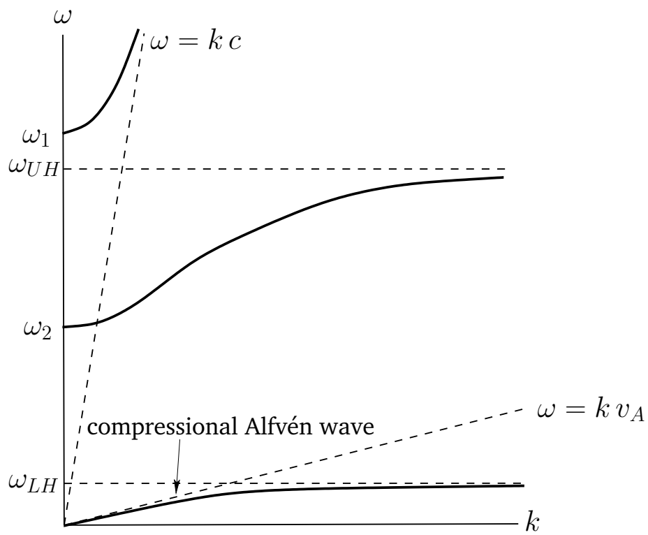
Figure 14: Dispersion relation for a wave propagating perpendicular to the magnetic field in a magnetized plasma.
