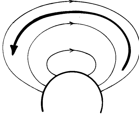
Figure 12: Typical path of a whistler wave through the Earth's magnetosphere.
