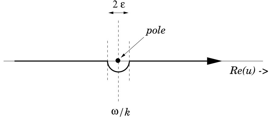
Figure 34: Integration path about a pole.
