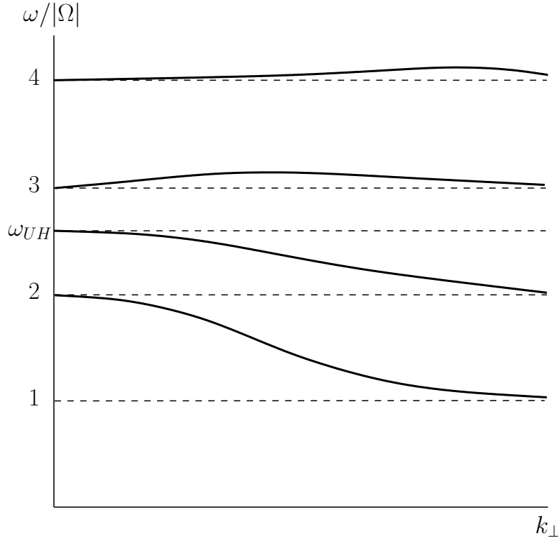
Figure 38: Dispersion relation for electron Bernstein waves in a warm plasma.
