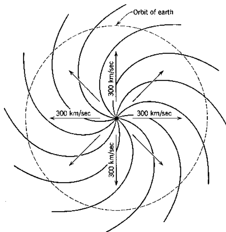
Figure 19: The interplanetary magnetic field.
