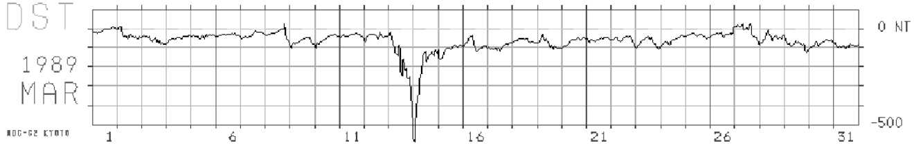
Figure 3: Dst data for March 1989 showing an exceptionally severe geomagnetic storm on the 13th.
