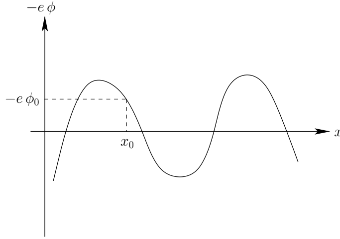
Figure 35: Wave-particle interaction.
