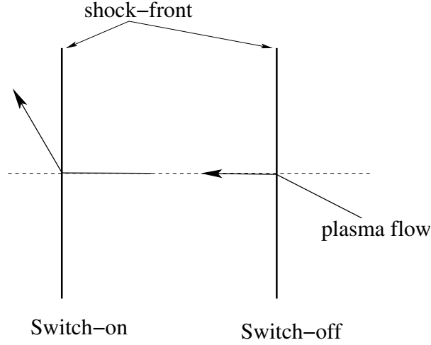
Figure 30: Characteristic plasma flow patterns across switch-on and switch-off shocks in the shock rest frame.
