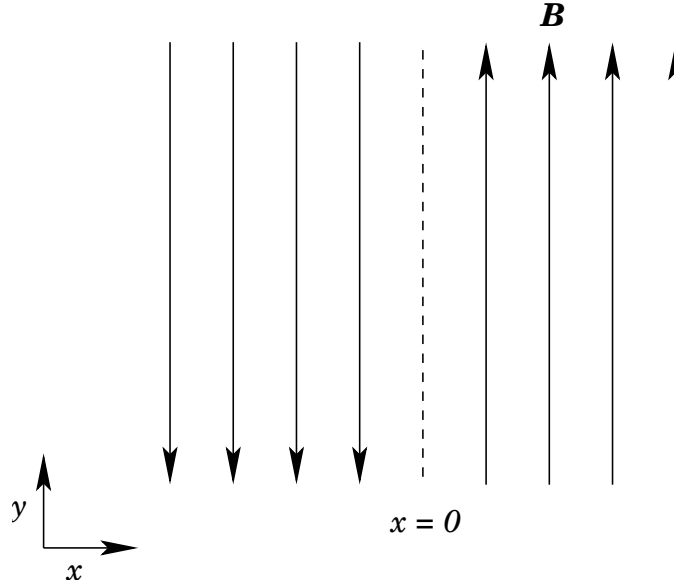
Figure 24: A reconnecting magnetic field configuration.
