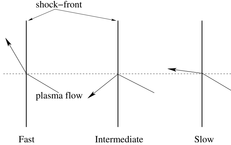
Figure 29: Characteristic plasma flow patterns across the three different types of MHD shock in the shock rest frame.
