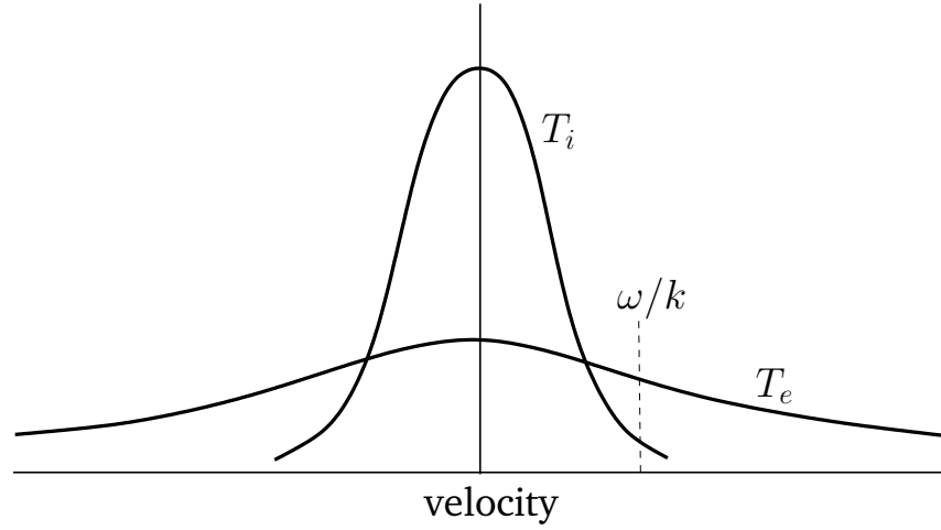
Figure 37: Ion and electron distribution functions with T_i \ll T_e .
