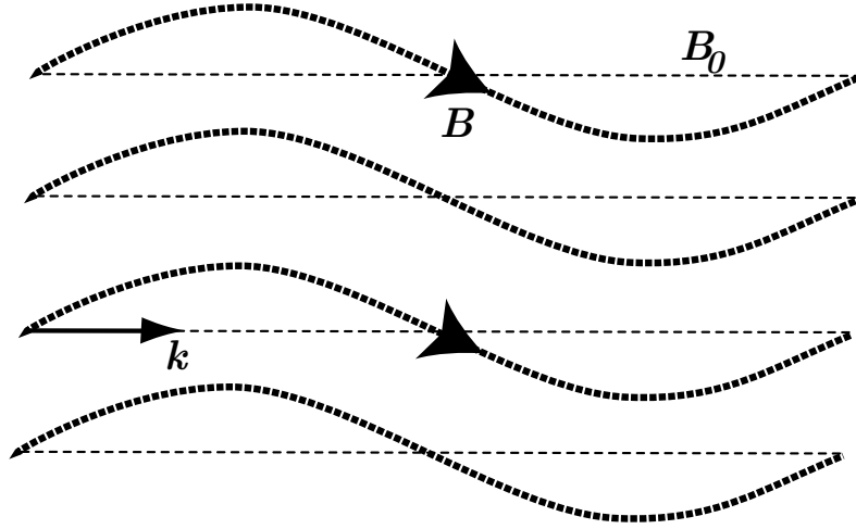
Figure 8: Magnetic field perturbation associated with a shear-Alfvén wave.
