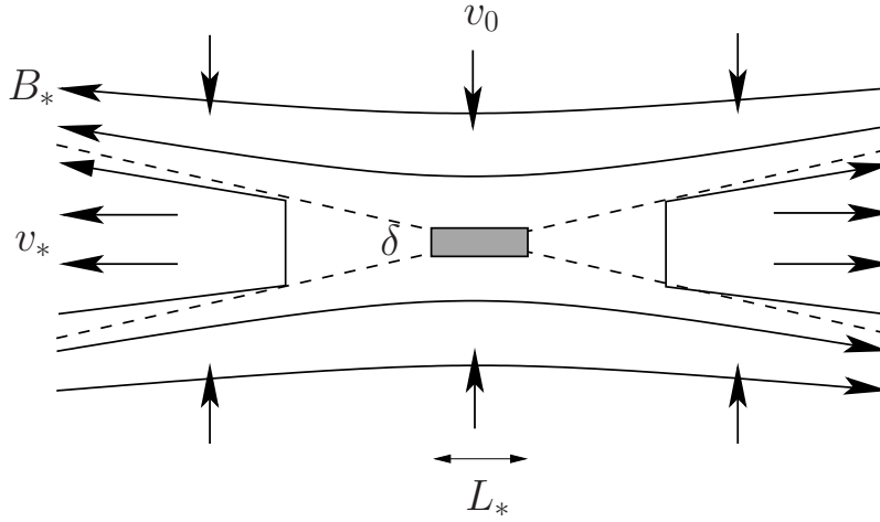
Figure 27: The Petschek magnetic reconnection scenario.
