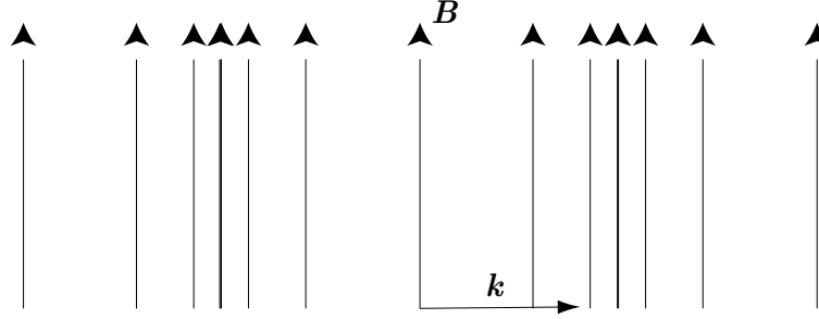
Figure 9: Magnetic field perturbation associated with a compressional Alfvén-wave.
