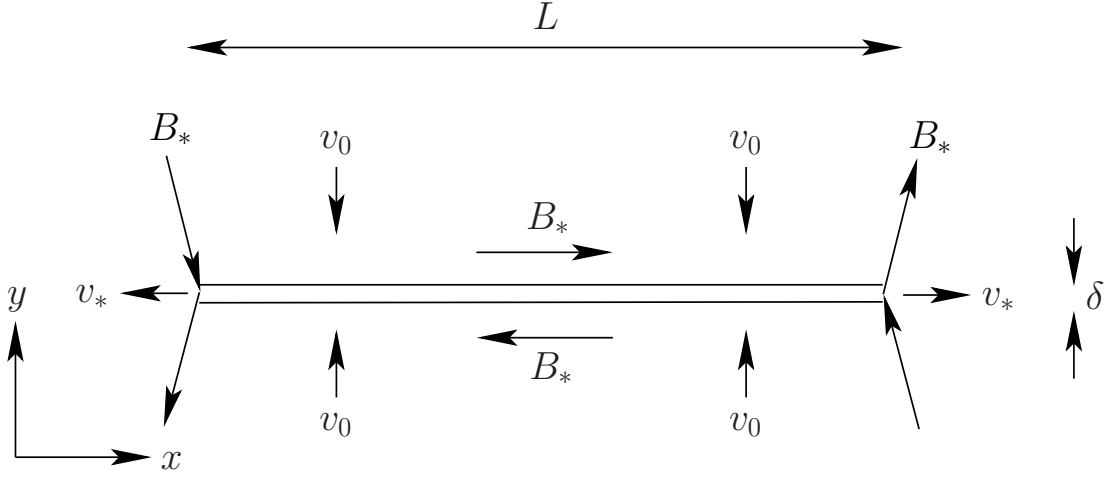
Figure 26: The Sweet-Parker magnetic reconnection scenario.
