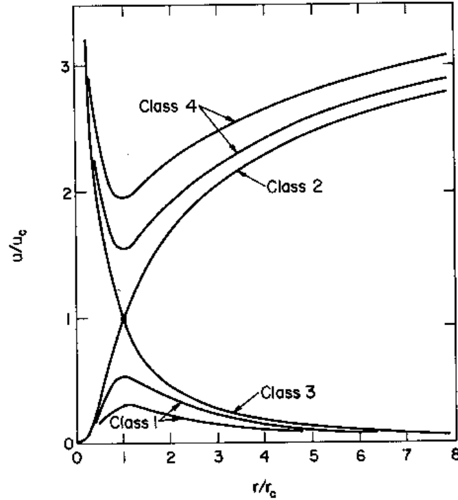
Figure 17: The four classes of Parker outflow solutions for the solar wind.
