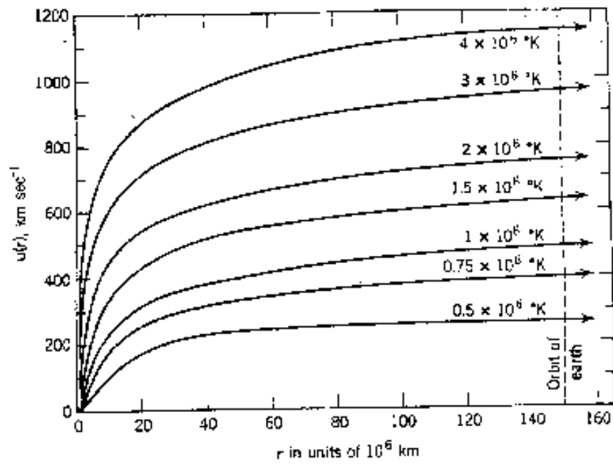
Figure 18: Parker outflow solutions for the solar wind.
