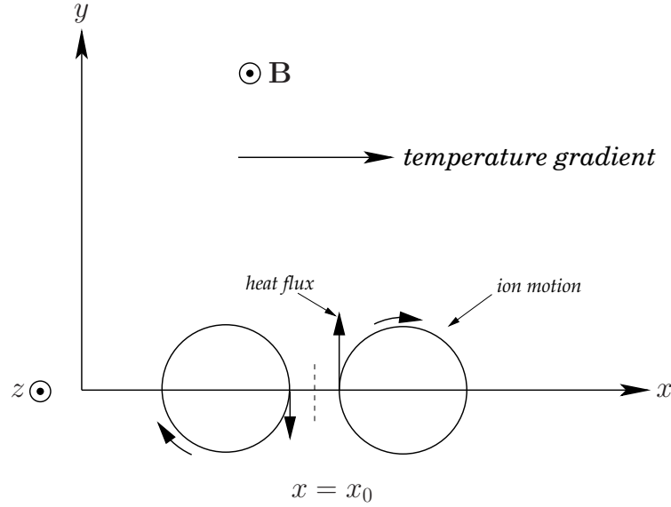
Figure 6: Origin of the convective perpendicular heat flux in a magnetized plasma.
