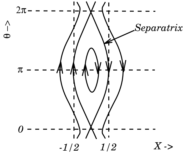
Figure 25: Magnetic field-lines in the vicinity of a magnetic island.
