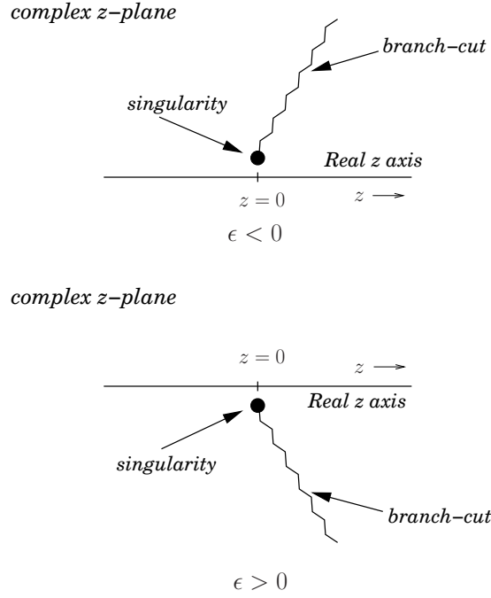
Figure 15: Branch-cuts in the z -plane close to a wave resonance.
