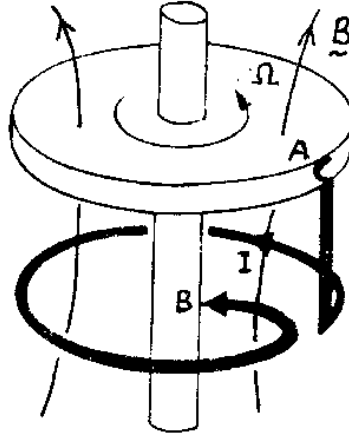
Figure 22: The homopolar generator.
